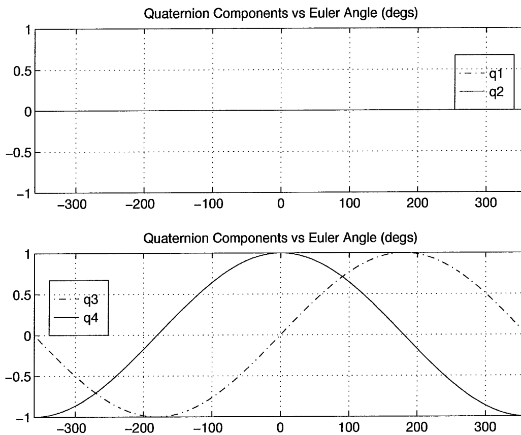
Figure 4. Quaternions for Pitch Only Rotation
