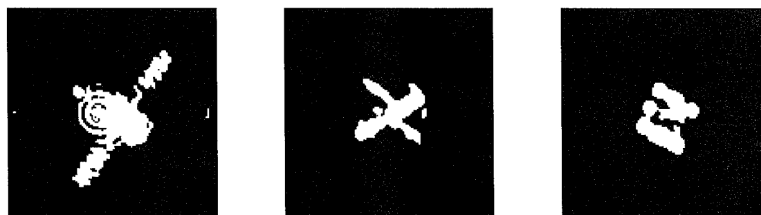
Binary images
