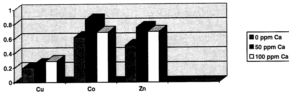
Figure 4-14 Normalized Metabolic Activity as a Function of Calcium Concentration The inhibition of metals decreases as Ca is increased from 0 to 50 ppm but the inhibition increases as calcium is increased from 50 to 100 ppm for cobalt and zinc
