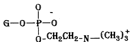
Choline phosphoglyceride
