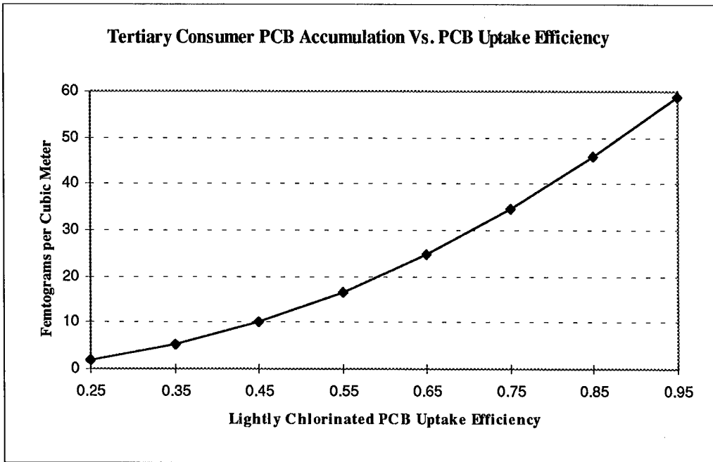
Tertiary Consumer PCB Accumulation Vs. PCB Uptake Efficiency (The PCB Uptake Efficiency on Figure 32 is for lightly chlorinated PCBs. The PCB Uptake Efficiency for heavily chlorinated PCBs is .1 less than the lightly chlorinated PCB Uptake Efficiency.)
