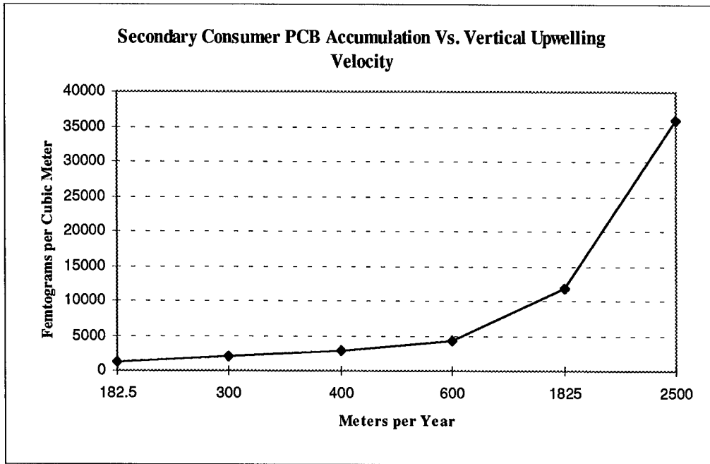
Secondary Consumer PCB Accumulation Vs. Vertical Upwelling Velocity
