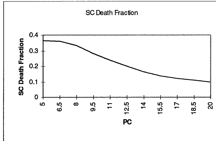
SC Death Fraction Vs. PC
