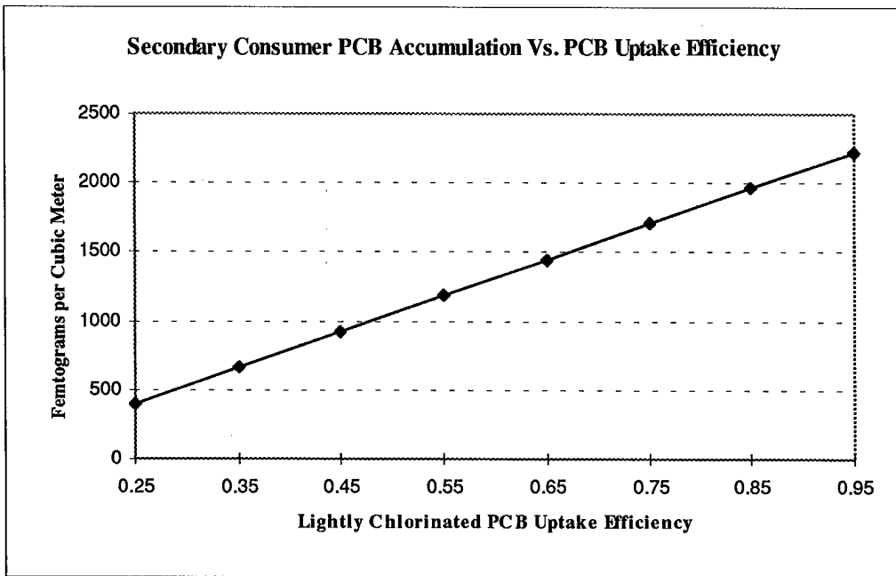
Secondary Consumer PCB Accumulation Vs. PCB Uptake Efficiency (The PCB Uptake Efficiency on Figure 33 is for lightly chlorinated PCBs. The PCB Uptake Efficiency for heavily chlorinated PCBs is .1 less than the lightly chlorinated PCB Uptake Efficiency.)
