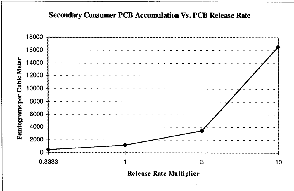
Secondary Consumer PCB Accumulation Vs. PCB Release Rate Multiplier
