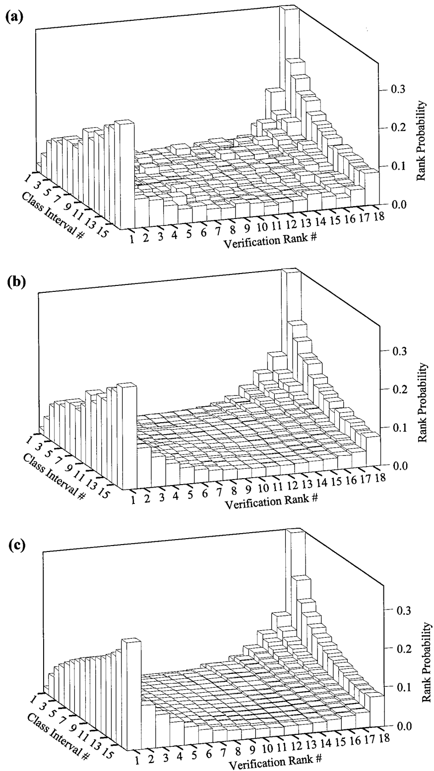
Figure 19. Processing of verification rank histograms for 2.5-day forecasts. (a) Raw data with noise in both directions. (b) After smoothing between the ranks at each class interval of standard deviation. (c) After fitting third-order polynomials at each rank.
