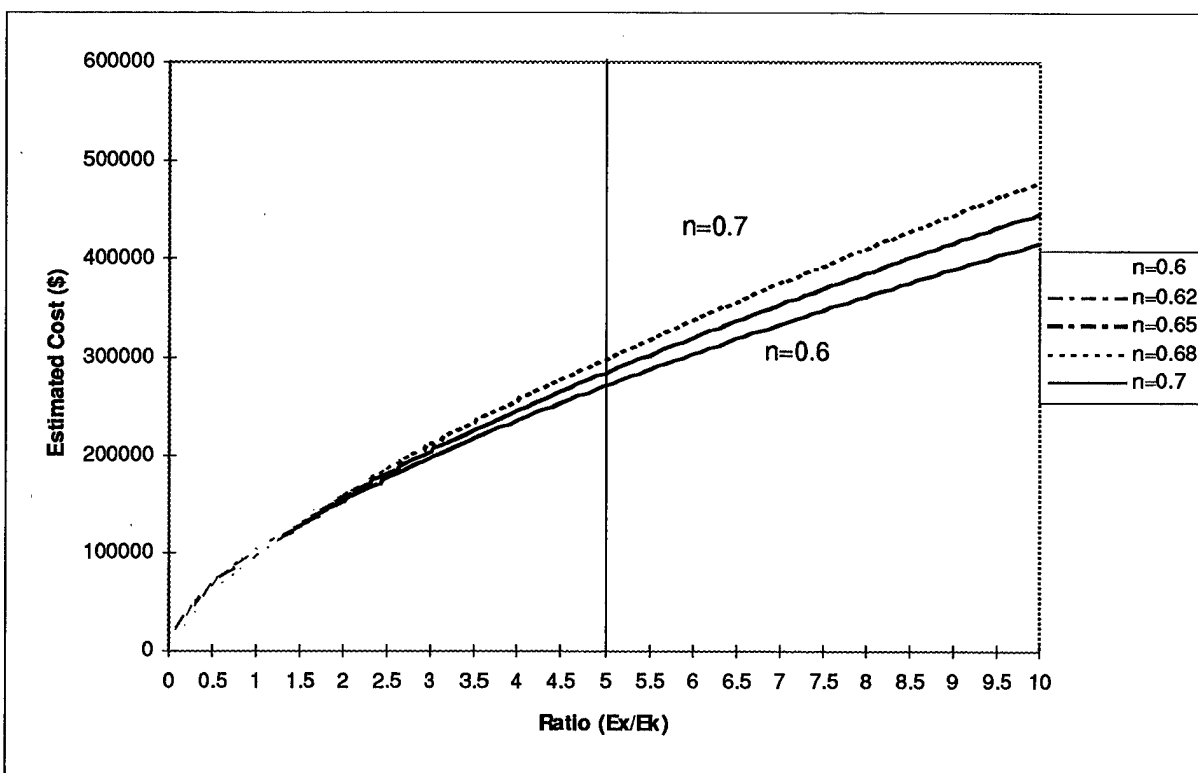
Figure 2-8 Six-Tenth Rule
