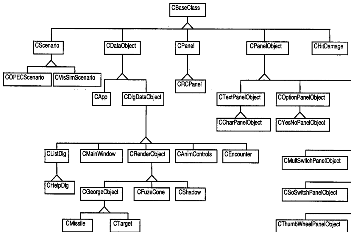
Figure 4-8: Class Hierarchy
