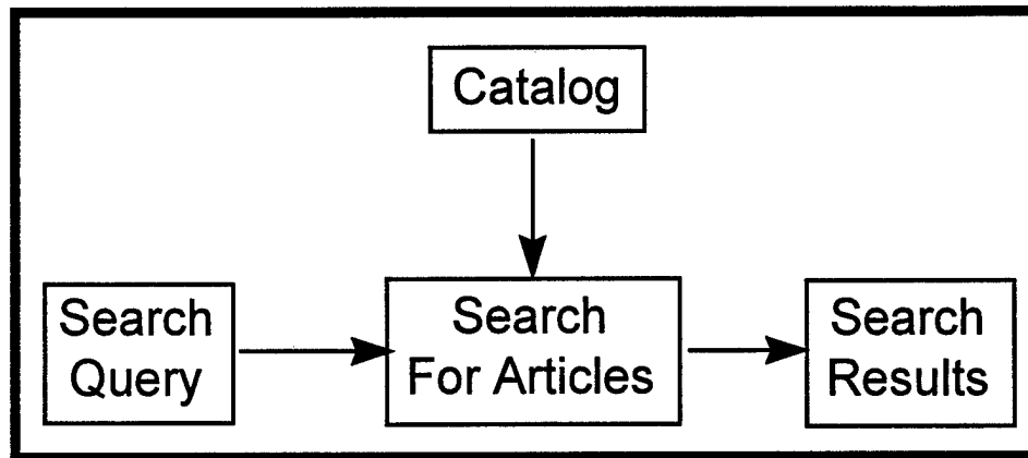
Figure 3. Query Process
