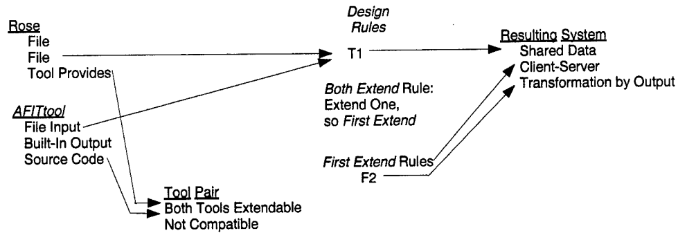
Figure 8 Rose/AFITtool Integration
