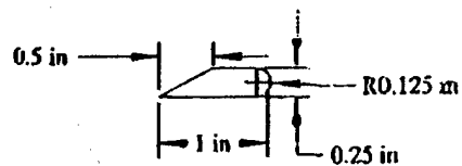
Chord for 60° Swept Wing
