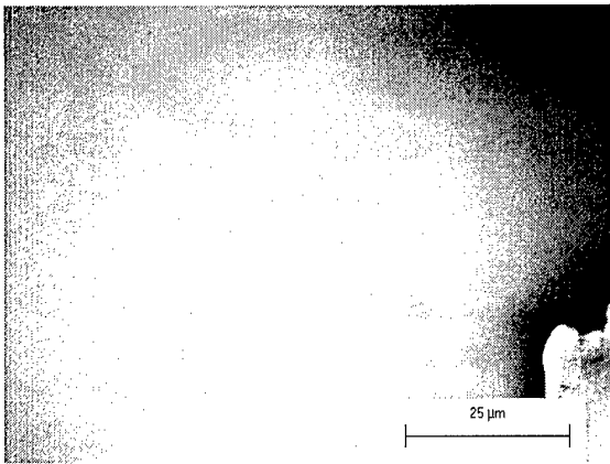
Wafer 6 – Trench 4 at 1000x magnification – post 2-hour polish, pressure = 11 lb/in 2 , rpm = 90 condition
