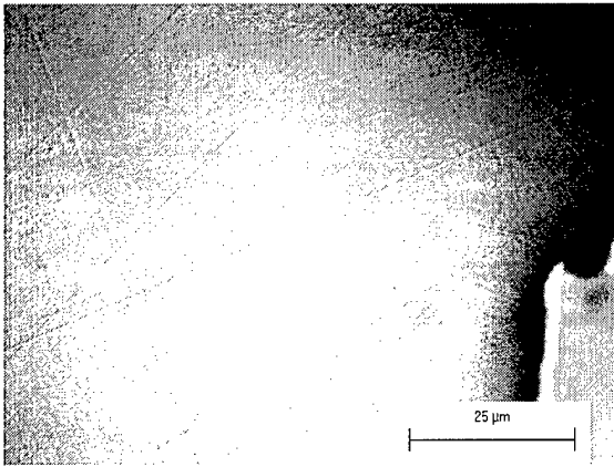
Wafer 6 – Trench 4 at 1000x magnification – pre-polish, pressure = 11 lb/in 2 , rpm = 90 condition
