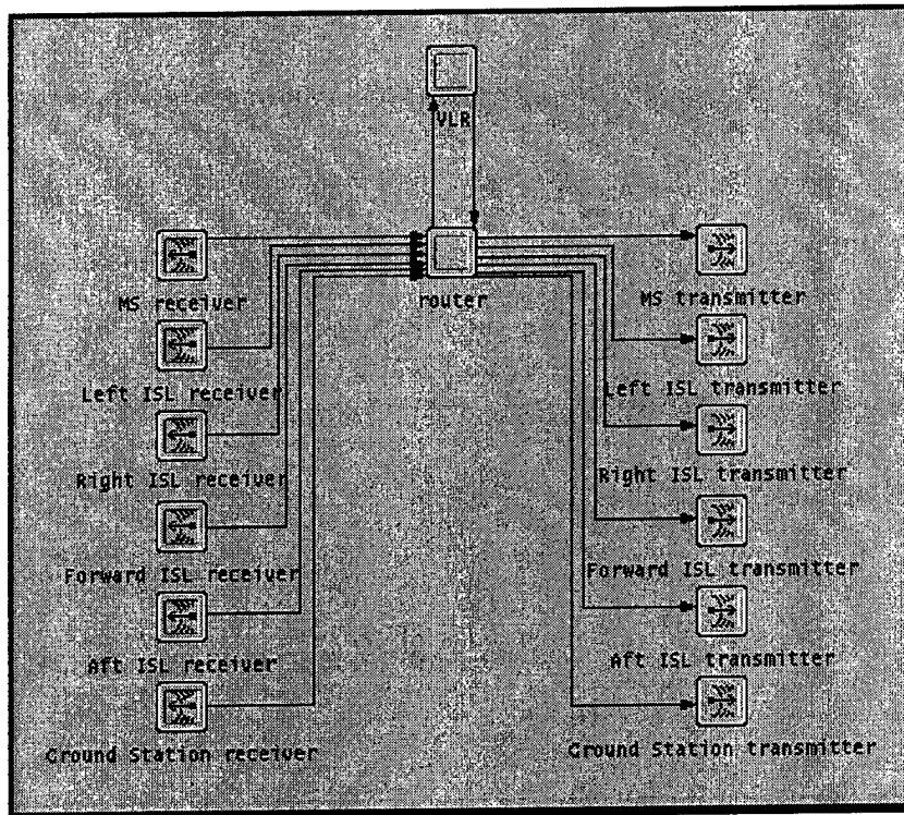
Figure 16. The Enhanced Iridium ® Satellite Model
