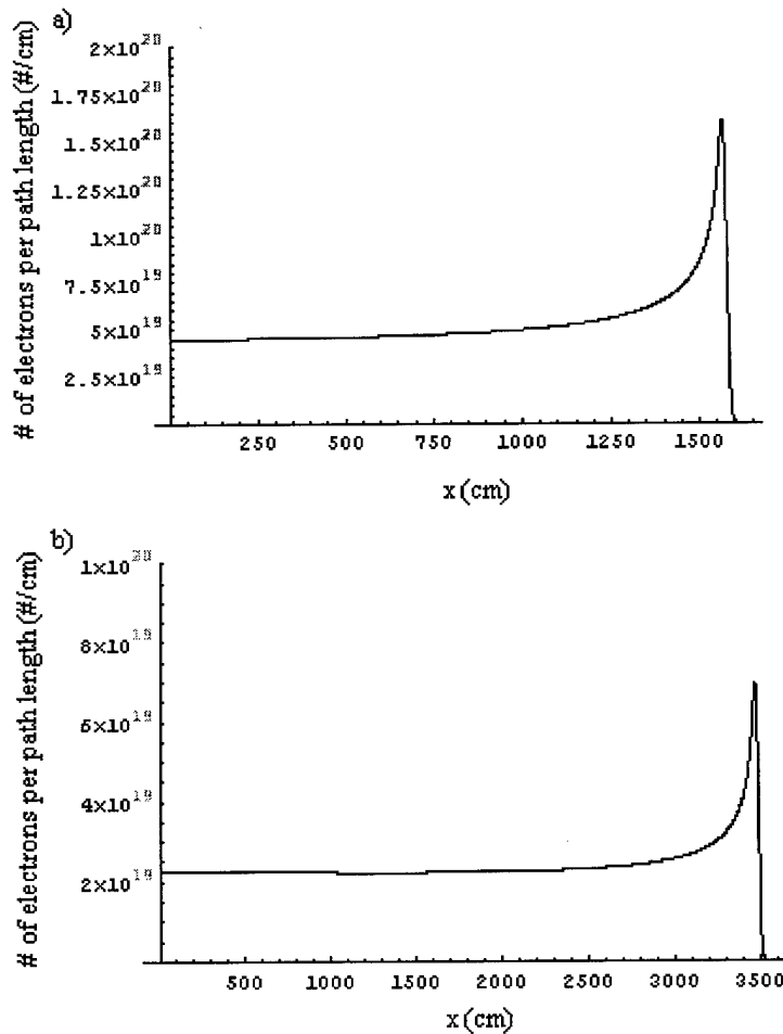
Figure 19. Electron Longitudinal Density Profile from the RNE Scenario for an Electron Beam of a) 1 MeV b) 2 MeV
