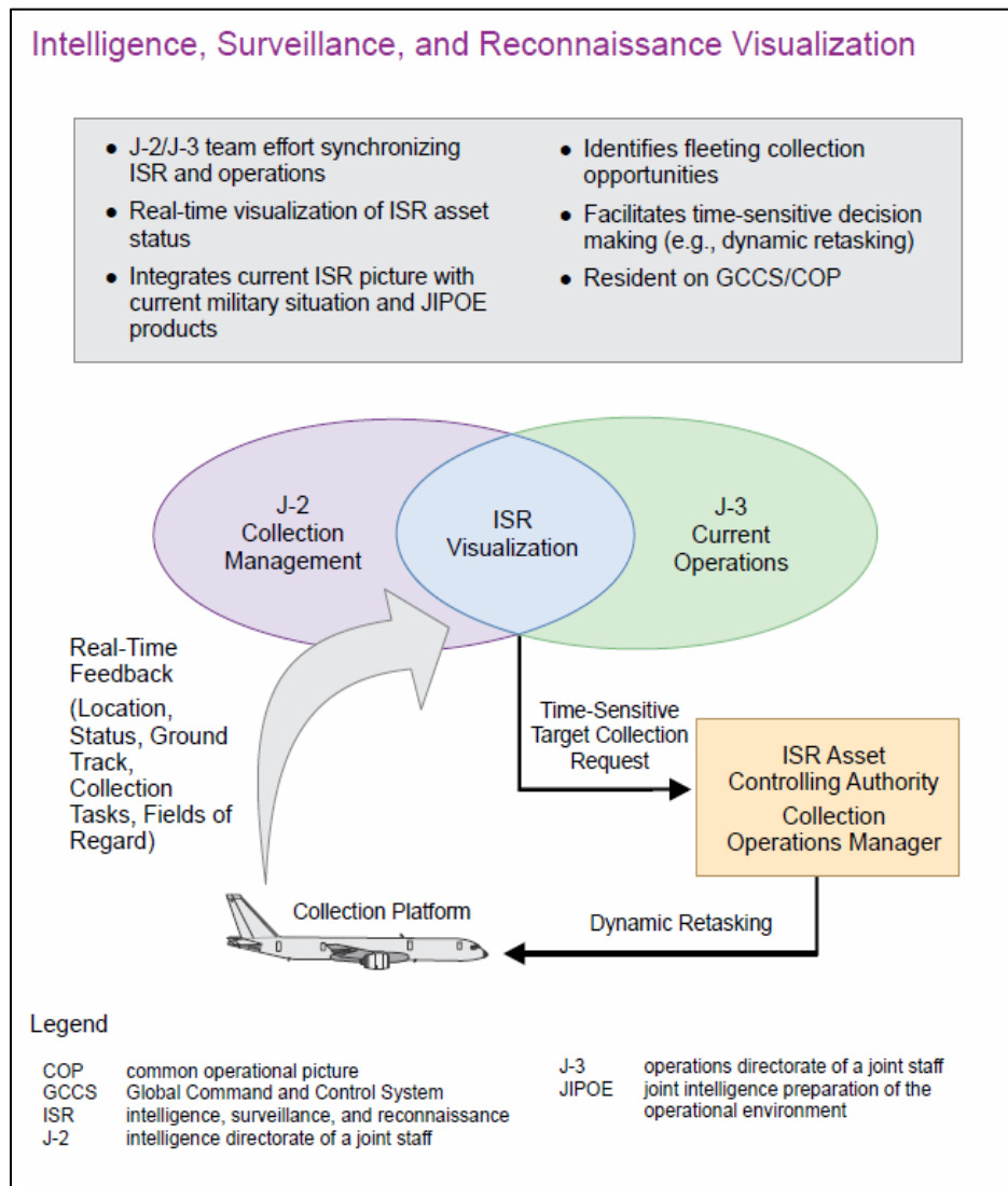
Figure 5. ISR Visualization
