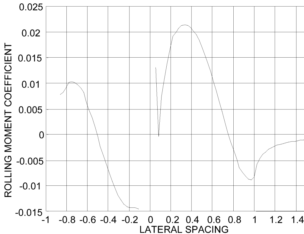
Figure 2-10. Rolling Moment of #3 Wingman
