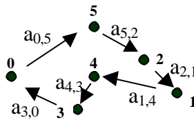
Figure 3.1 Cyclic Digraph Example
