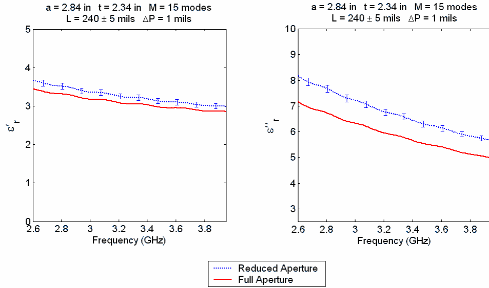
Figure 4-9. Permittivity of ERAM test sample mounted flush toward port two in the 2.34-inch sample holder. Maximum difference of real/imaginary permittivity is 6.55/14.02% relative to their full-aperture baselines, without considering thickness and placement uncertainties. (Permittivity only extraction using all four S-parameters.)
