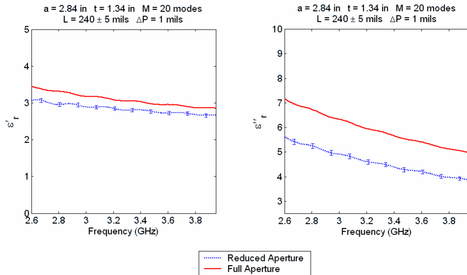
Figure 4-10. Permittivity of ERAM test sample mounted flush toward port two in the 1.34-inch sample holder. Maximum difference of real/imaginary permittivity is 11.01/22.71% relative to their full-aperture baselines, without considering thickness and placement uncertainties. (Permittivity only extraction using all four S-parameters.)
