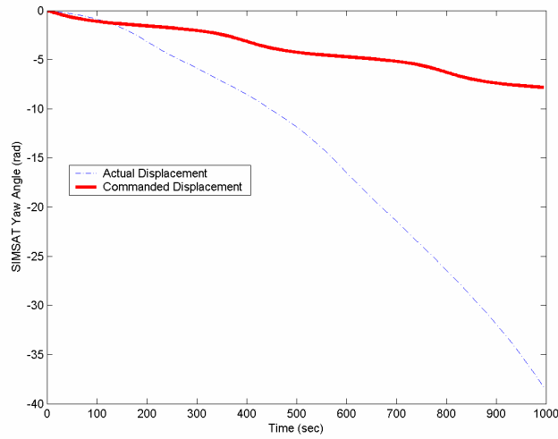
Figure 17. Initial Measurements of SIMSAT Body Yaw Rate with Forced \dot{\hat{\mathbf{b}}}
