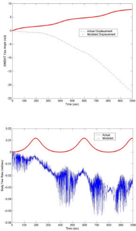
Figures 19. SIMSAT Yaw Angle and Rate vs. Time (Positive Case)
