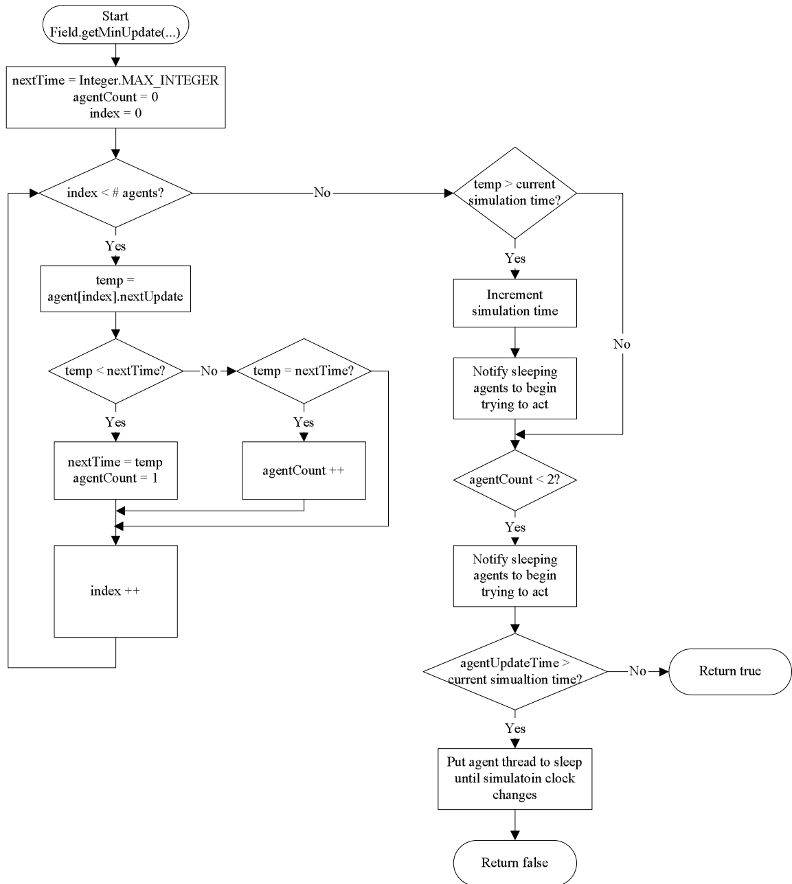
Figure B.7 Field getMinUpdate Method Algorithm Used to Advance the Simulation Clock and Control Agent Timing
