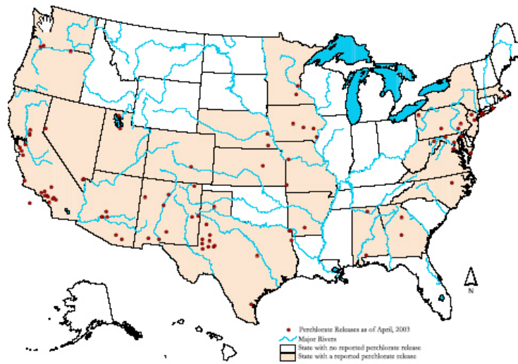
Figure 2.2 Map of perchlorate releases. Shading indicates states with reported perchlorate releases. Dots indicate specific release locations (Mayer, 2004b)
