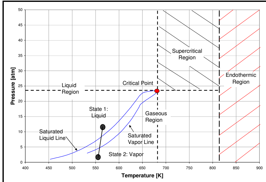
Figure 12. Representative pressure vs. temperature diagram for a typical low vapor pressure fuel
