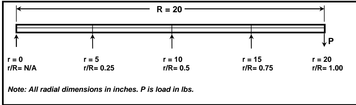
Figure 2: Side-view of Beam #2
