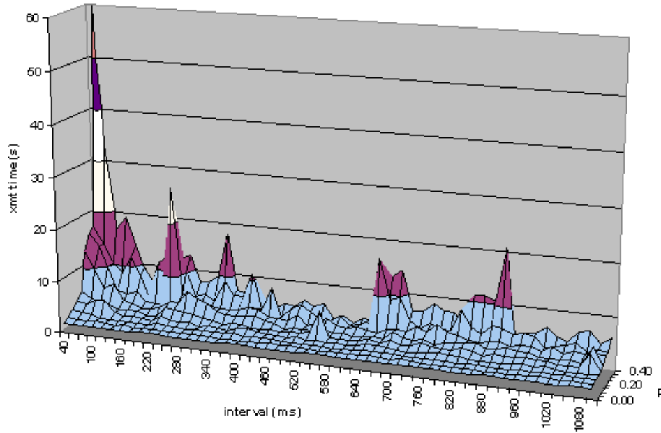
Figure 4.8: Average observed time of file transmission plotted for link wink probability and interval length using Hybla congestion control algorithm.
