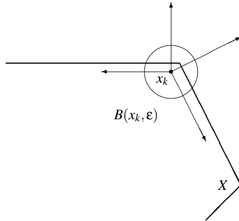
Figure 3.3: Directions that Conform to the Geometry of X
