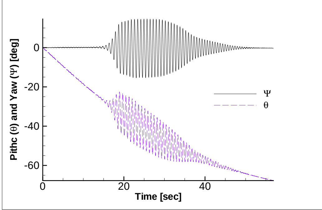
Figure 41: Extended Orientation History of MK-84 AIR at Mach 0.9 at 10,000 ft
