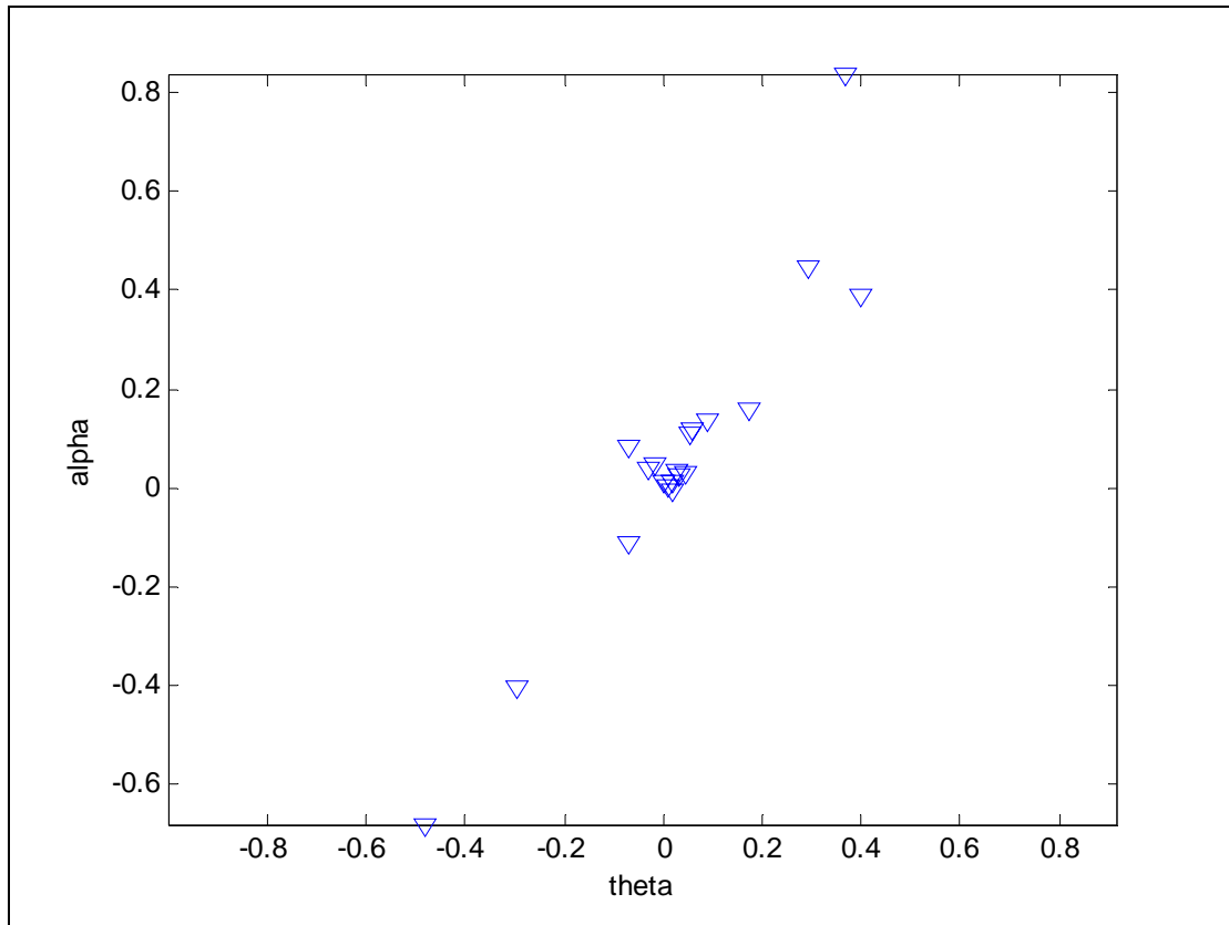
Figure 5-12: Rotation-Deformation angles
