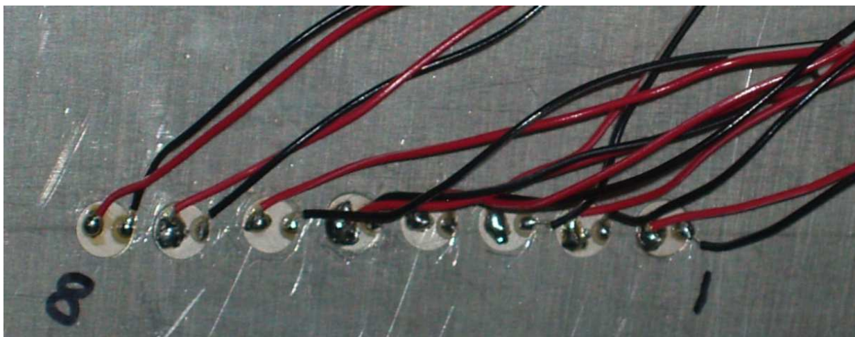
Figure 2.9 MPP: array of middle APC 850 piezos
