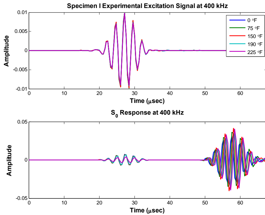
Figure 104: Specimen I Raw Signals at 400 kHz Specimen I Experimental S_0 Response at 400 kHz
