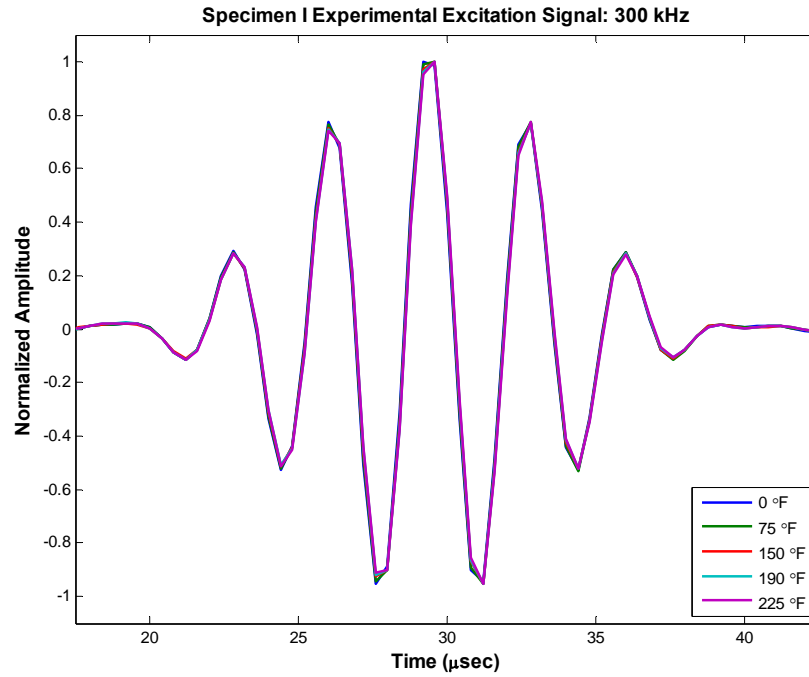
Figure 40: Specimen I Experimental Excitation Signals at 300 kHz
