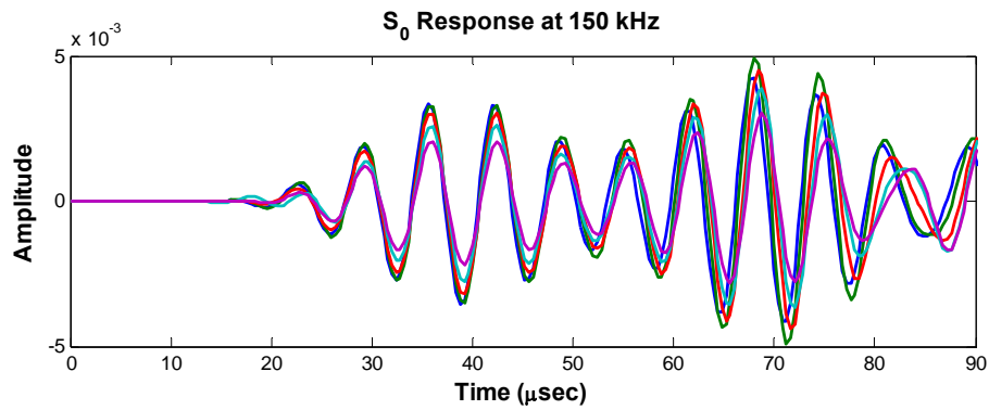
Figure 96: Specimen I Raw Signals at 150 kHz
