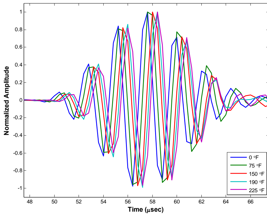
Figure 105: Specimen I Experimental S_0 Response at 400 kHz
