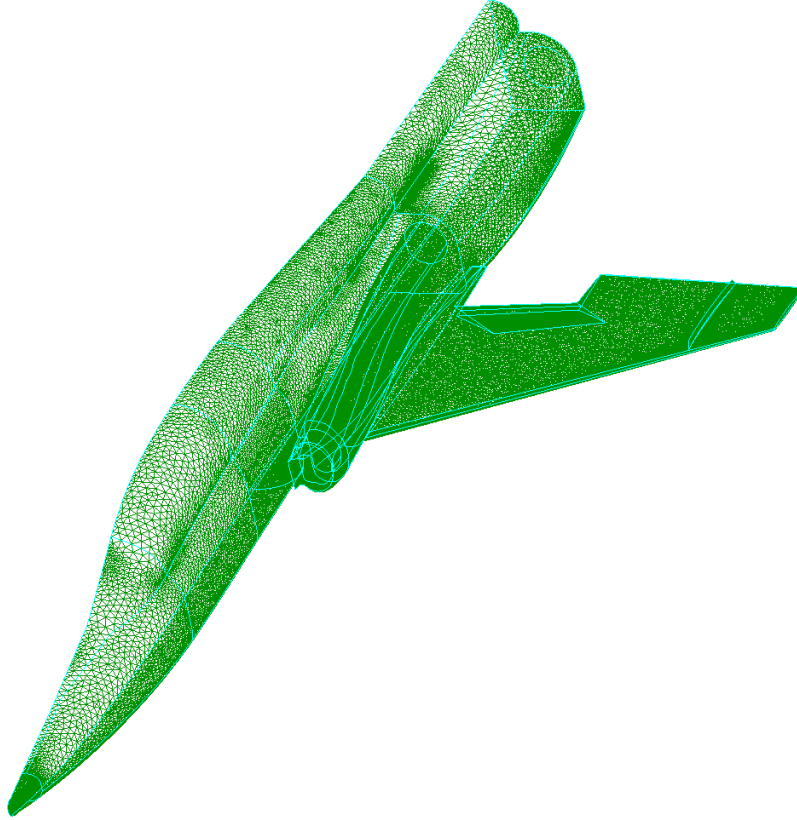
Figure 3.4: Baseline surface mesh with a simple fence.
