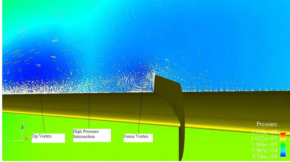
Figure 4.5: Extended fence vortices at 15° AOA.
