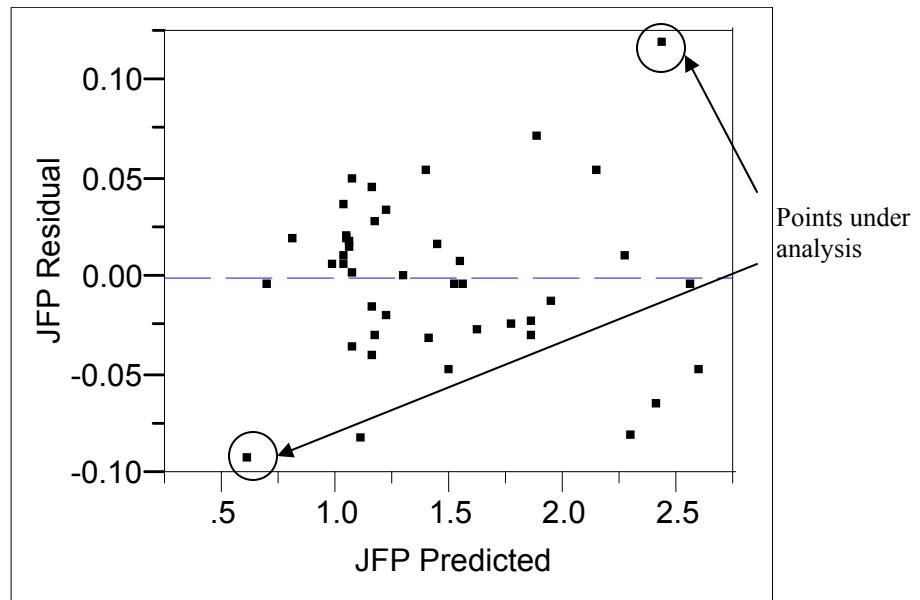
Figure 4.6: Residuals' Scatterplot
