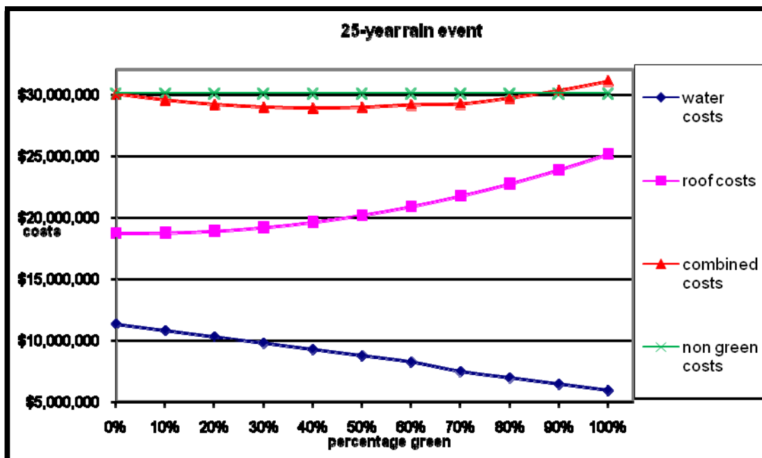
Figure 4.1: 25-year Rain Event Cost Curves
