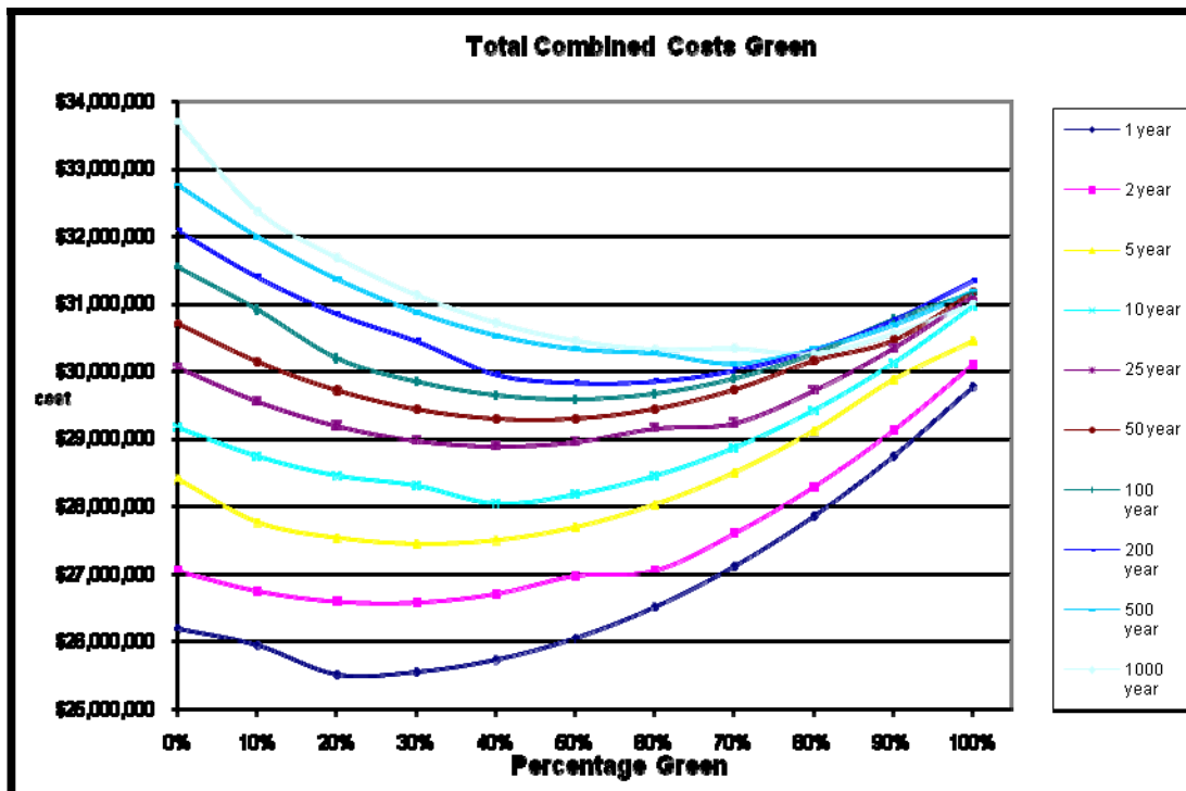
Figure 4.2: Overall graph of curves for costs verses rain events.
