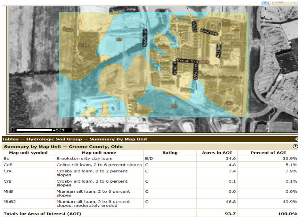
Figure 3.5: Hydrologic Soil group report from USDA for AOI
