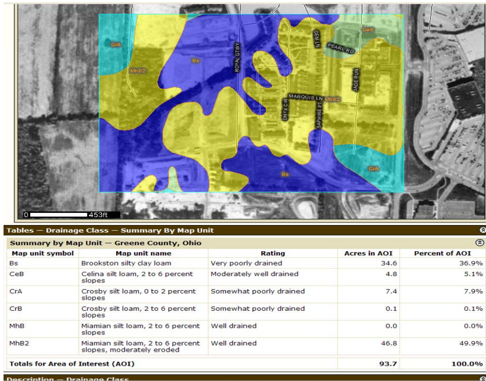
Figure 3.4: Soil types from USDA report for Area of Interest (AOI)
