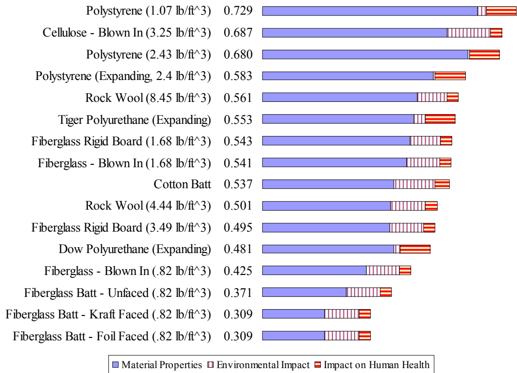
Figure 4.1. Climate Zone 1 Rankings – Second Tier (Minot, North Dakota)
