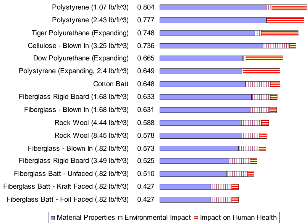
Figure 4.5. Climate Zone 5 Rankings – Second Tier (Niceville, Florida)
