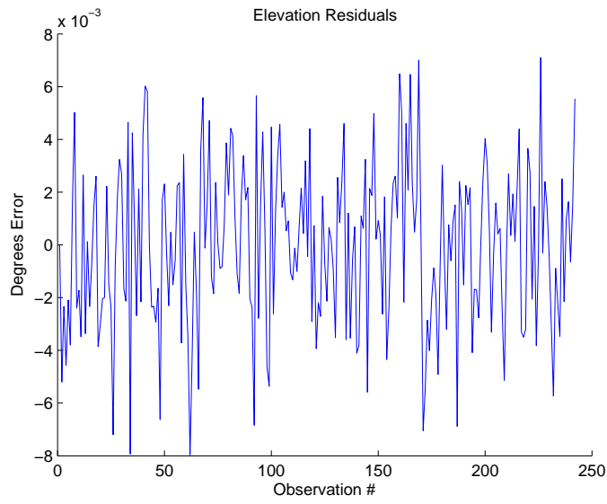
Figure A.8: Elevation Residuals With 3.18 \times 10^{-3} Noise for ISS
