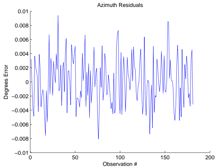
Figure A.9: Azimuth Residuals With 3.18 \times 10^{-3} Noise for N2 RB
