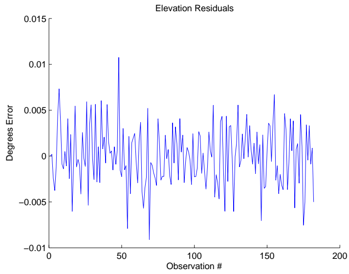
Figure A.10: Elevation Residuals With 3.18 \times 10^{-3} Noise for N2 RB
