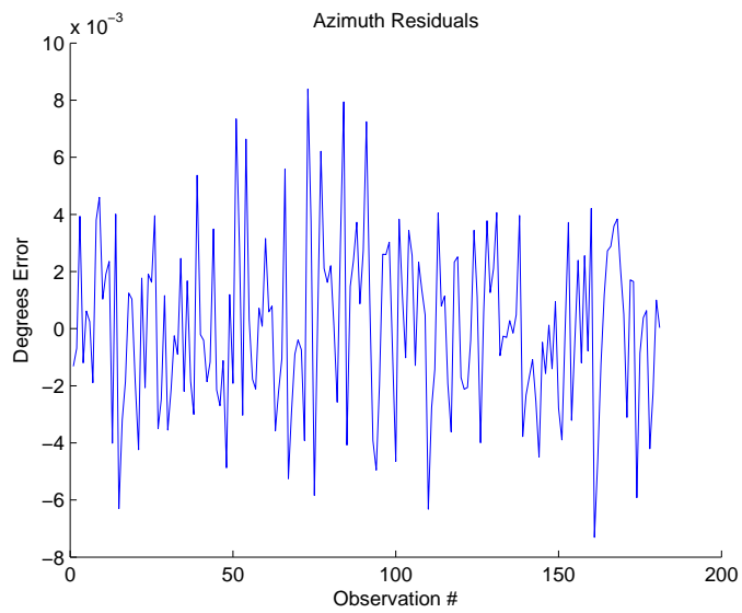
Figure A.11: Azimuth Residuals With 3.18 \times 10^{-3} Noise for ISS
