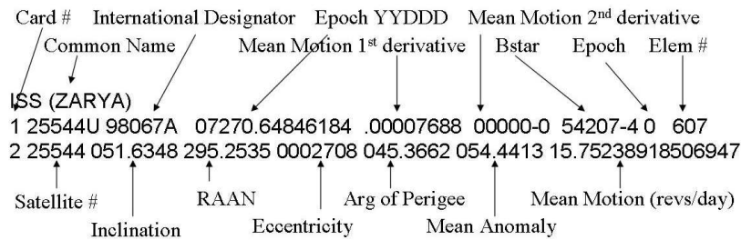
Figure 2.3: Two Line Element Set
