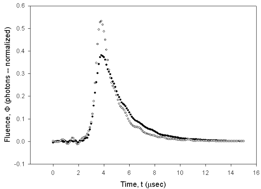
Figure 4.2: Sample normalized time-of-flight flux curves for Ba ( \bullet ) and Cu ( \circ ) neutral emission. Ba I was collected with a narrowband spectral filter centered at 767 nm, while Cu I was collected with a similar filter at 809 nm. Cu peak flux is more narrowly peaked than Ba. Data collected at 150 mTorr and 36.00 mm downstream of target. Flux curves are normalized such that the area under the curve is equal to one.
