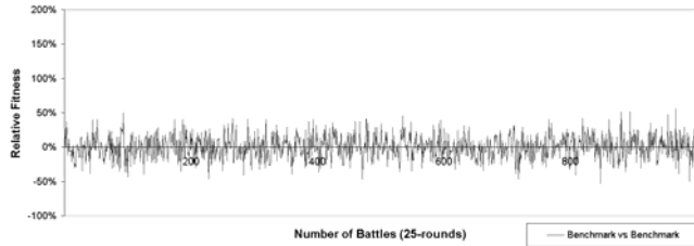
Figure 4b: Noise for Benchmark vs. Benchmark (25-rounds).
