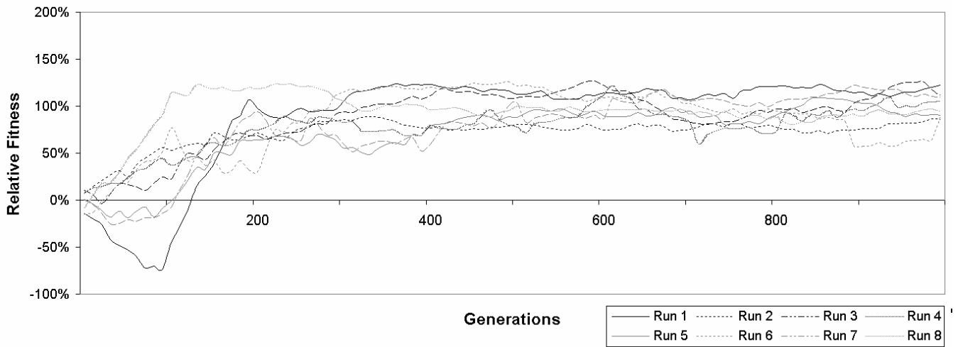
Figure 5a: Progression of eight individual populations, measured relative to the benchmark.
