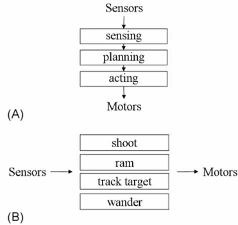
Figure 1: Two organization decompositions for robot control (A) Sequential execution of functional modules; (B) A task-based decomposition into parallel execution modules.
