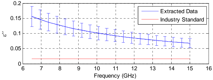
Figure 40: Relative complex permittivity of 4.39 mm thick Plexiglas sample with Blackman-Harris Windowing using 6" and 4" square flange plates
