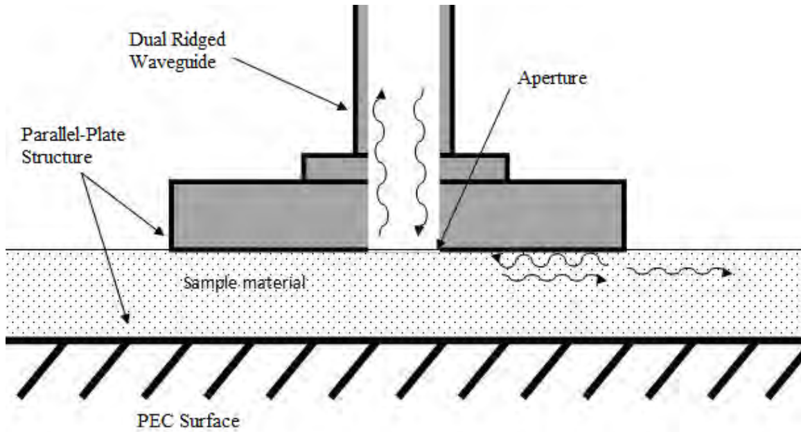
Figure 1: Basic setup of probe
