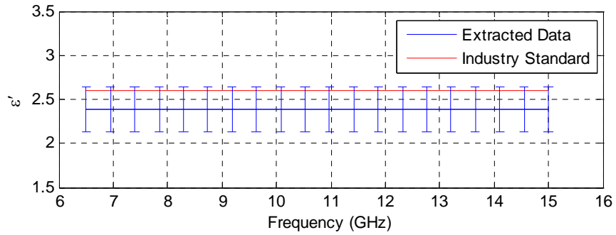
Figure 39: Relative complex permittivity of 5.55 mm thick Plexiglas sample with Blackman-Harris Windowing using 6" and 4" square flange plates
