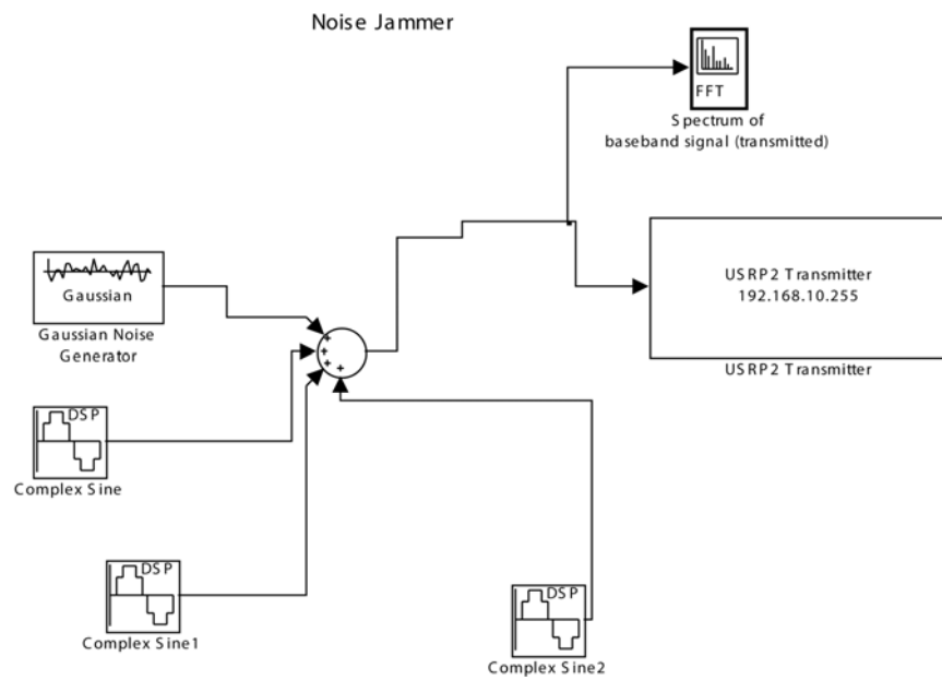
Figure 3.9: Simulink diagram showing the configuration for the USRP2 noise jammer.
