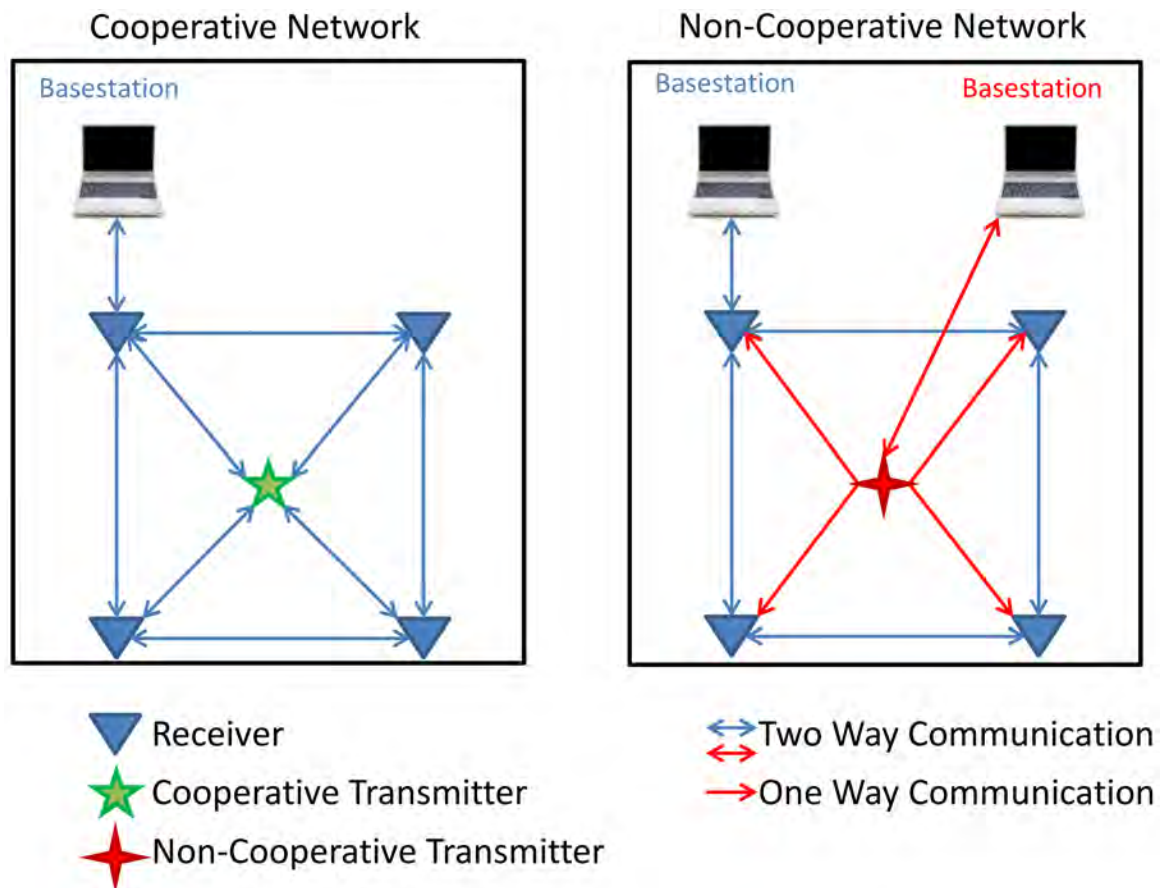
Figure 1.1: Diagram showing the difference between a Cooperative Network and Non-Cooperative Network [3].
