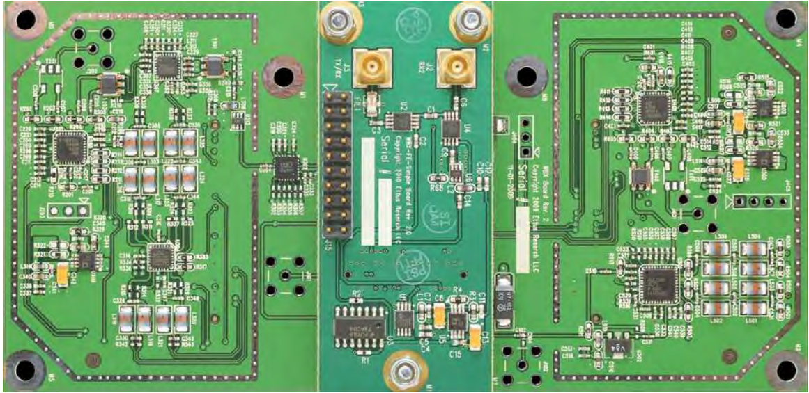
Figure 2.2: WBX Daughterboard [8].
