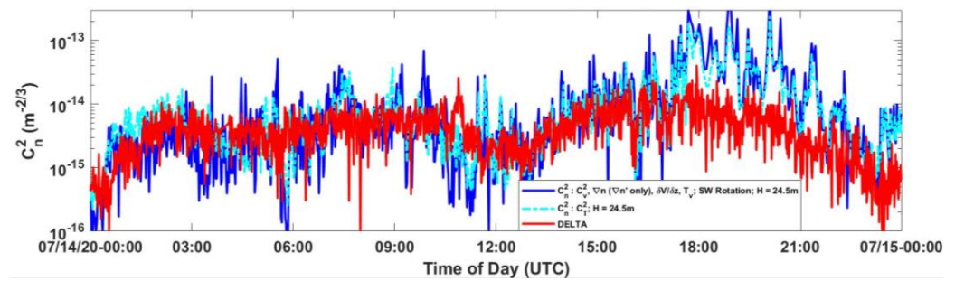
Figure 9. Profiles of C_n^2 at 24.5 above the surface using in situ sonic anemometer measurements (derived from C_n^2 , \nabla \langle n' \rangle , \frac{\partial \langle V \rangle}{\partial z} , mean = 1.3 \times 10^{-14} , std dev = 3.6 \times 10^{-14} ) as well as the DELTA system (mean = 4.8 \times 10^{-15} , std dev = 3.4 \times 10^{-15} ). For comparison, a profile of C_n^2 at 24.5 m as derived from C_T^2 (mean = 9.8 \times 10^{-15} , std dev = 1.9 \times 10^{-14} ) on 14 July 20 at Wright-Patterson AFB.
