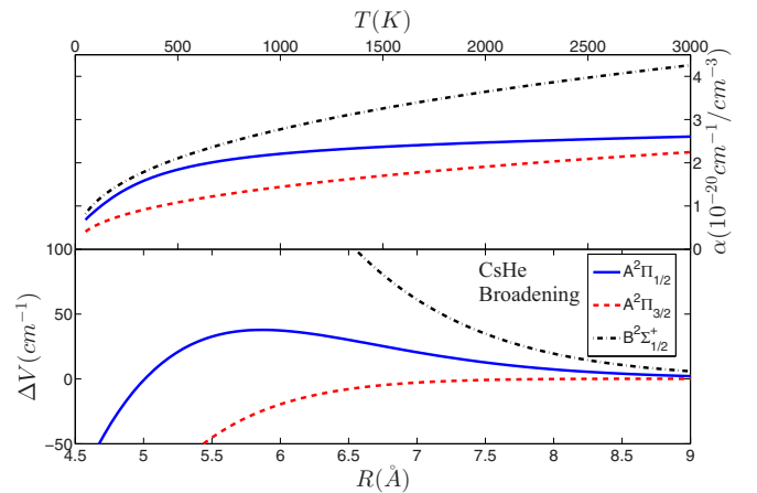
FIG. 10. (Color online) The Cs + He \Delta V_{\Pi_{1/2}} , \Delta V_{\Pi_{3/2}} , and \Delta V_{\Sigma_{1/2}} DPs are plotted on the bottom and the corresponding broadening coefficients \alpha(T) are plotted on the top. The A^2\Pi_{3/2} and B^2\Sigma_{1/2}^+ broadening coefficients are plotted here separately. Their weighted average in Eq. (11) is used to compute the D_2 broadening coefficient.
