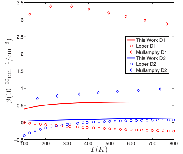
FIG. 19. (Color online) A comparison of Shifting coefficients computed using the semiclassical AT theory with other theoretical calculations. The Loper [22], Loper and Weeks [23], and Mullamphy et al. [19] calculations are described in Fig. 18.
