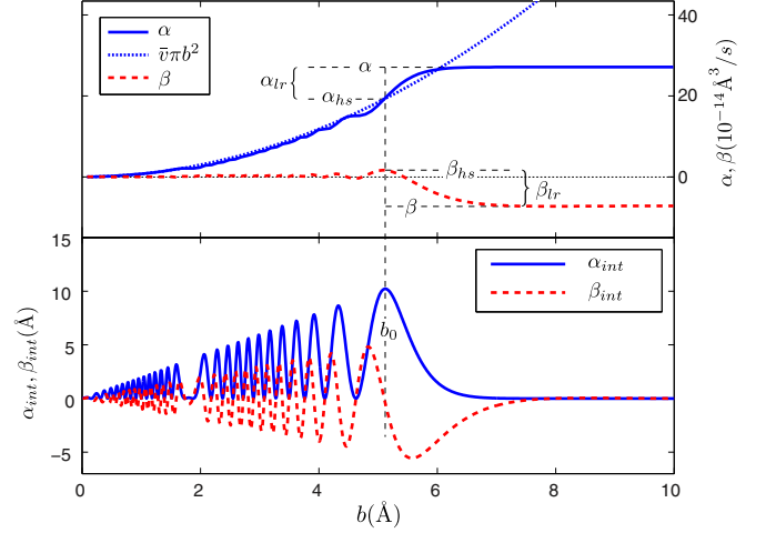
FIG. 5. (Color online) Integrands \alpha_{\text{int}} and \beta_{\text{int}} given by Eqs. (12) and (13) computed using the Cs + He \Delta V_{\Sigma_{1/2}} DP at \bar{v}(T = 1000 K) are plotted on the bottom. The integrals 2\pi\bar{v} \int_0^b db' \alpha_{\text{int}}(b') and 2\pi\bar{v} \int_0^b db' \beta_{\text{int}}(b') are plotted on the top and closely follow the effective hard-sphere values until b = b_0 .
