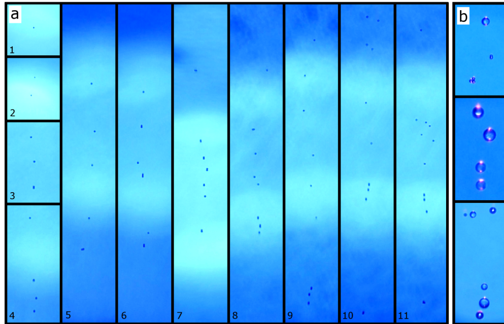
Fig. 2. Clustering of many particles as side viewed for 7 \mu\text{m} silica spheres suspended in air. (a) The number of particles grows from 1 to 11 as they keep falling (see Visualization 1 ). (b) Zooming-in reveals that multi-sized and multi-shaped particles can also optically bind. Red scattering is from a low-power probe beam (see Visualization 2 ). Scale bar is 50 \mu\text{m} in all images and beam waist is about 1 sphere diameter. With 11 particles the particle group center of mass was 240 \mu\text{m} above the beam waist.
