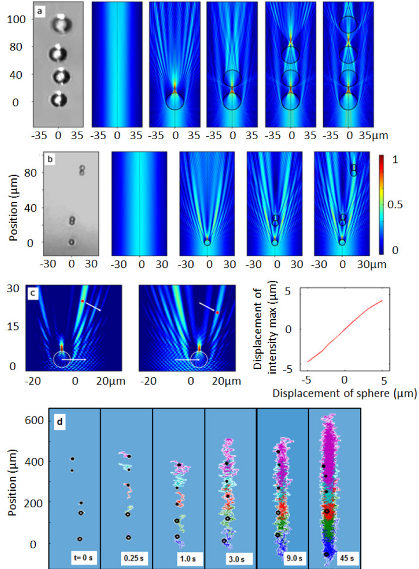
Fig. 4. Experimental results and modeling of (a) Silica microspheres, diameter 25 \mu\text{m} , 1D confined to a Gaussian beam trap (waist 0.8 microsphere diameters). Adding objects creates new intensity maxima, resulting in potential wells for trapping additional objects. (b) One spherical and two non-spherical objects in a weakly focused Gaussian beam (waist 4 microsphere diameters) trap where the structure turns 3D. (c) Long-range interaction of trapped particles. A 10 \mu\text{m} motion of a trapped particle results in a similar sized movement of the potential well at a distance of 4 diameters, or 18 wavelengths. (d) Dynamic simulation of trapped particles in an NA = 0.1 and 0.5 W, Gaussian beam where particle diameters from top to bottom are 5.6, 5.6, 7, 10.5 and 10.5 \mu\text{m} (see Visualization 5), as in the above experiment (Fig. 3.e).
