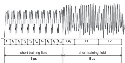
Fig. 1 Magnitude plot of first 16 \mu s of standard IEEE 802.11a physical layer preamble as received by USRP X310
