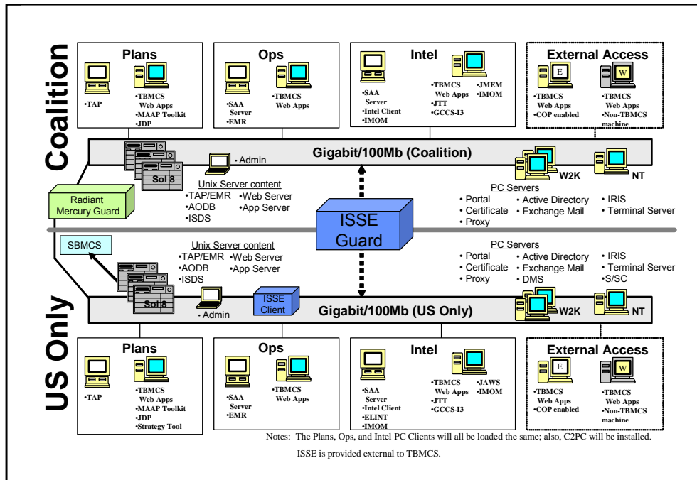
Figure 3-7. Physical/Hardware Architecture
